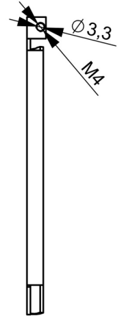
VIEW A
